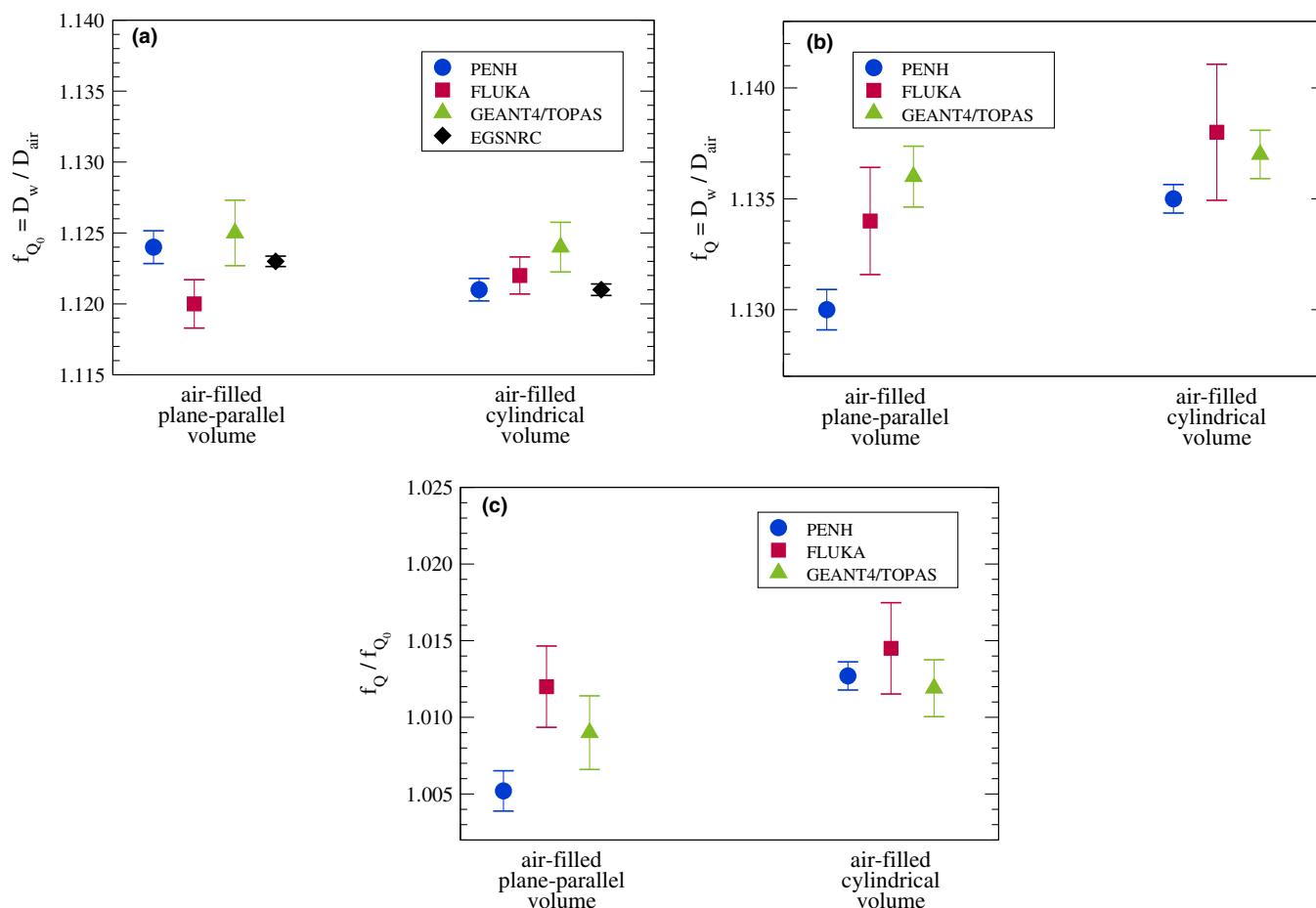
FIG. 3. Results for f_{Q_0} and f_Q factors: (a) 1.25 MeV photons and (b) 150 MeV protons. (c) The f_Q/f_{Q_0} ratios for 150 MeV protons. The statistical uncertainties represented by bars correspond to one standard deviation. [Color figure can be viewed at wileyonlinelibrary.com ]
