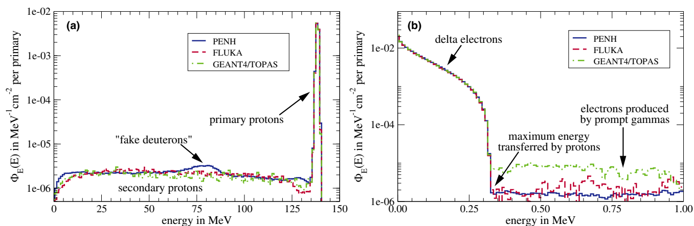
FIG. 5. Spectral fluence \Phi_E(E) in water of protons (a) and electrons (b) in the 150 MeV proton beam at a depth of 2 cm. [Color figure can be viewed at wileyonlinelibrary.com ]
